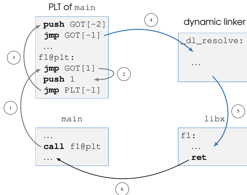
Figure B.3 – Control flow during the first call to f1
