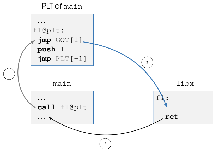
Figure B.4 – Control flow during the second and later calls of f1
