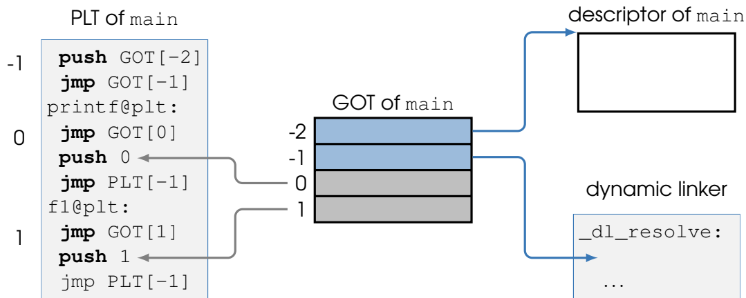
Figure B.2 – Initial arrangement of PLT and GOT in the example executable
